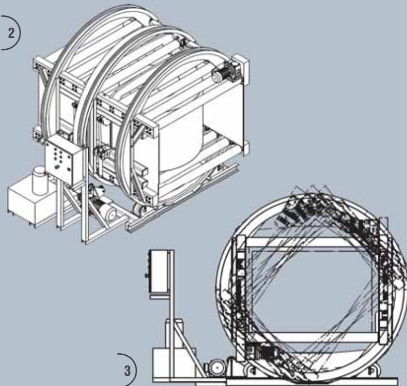
1-4 Elektromotorische Coilwendestation. Electromotive coil turning station.
